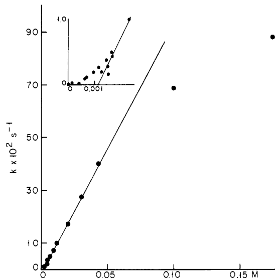
Figure 2. Plot of observed first-order constant vs. concentration of base for Fe(CO) 5 + base reaction. (Inset) expanded view of low base concentrations using buffer solutions.
